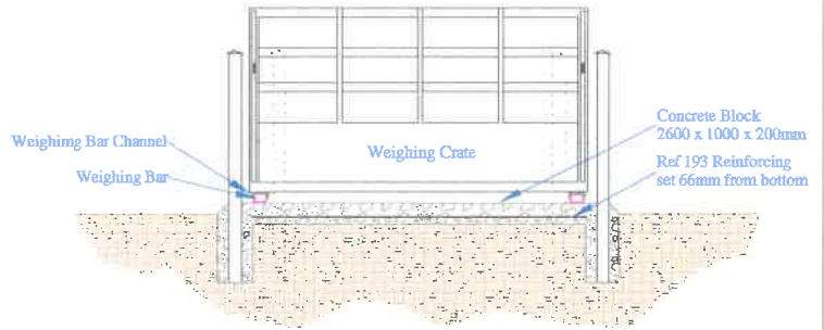
SIDE VIEW: WEIGHING CRATE
